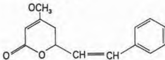
KAWAIN
